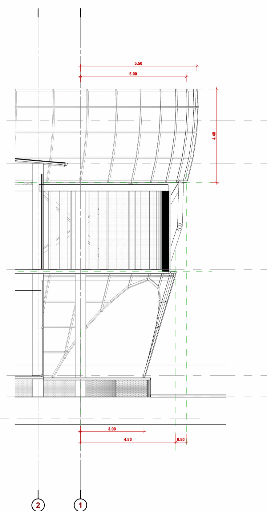
DETAIL - 3/5
