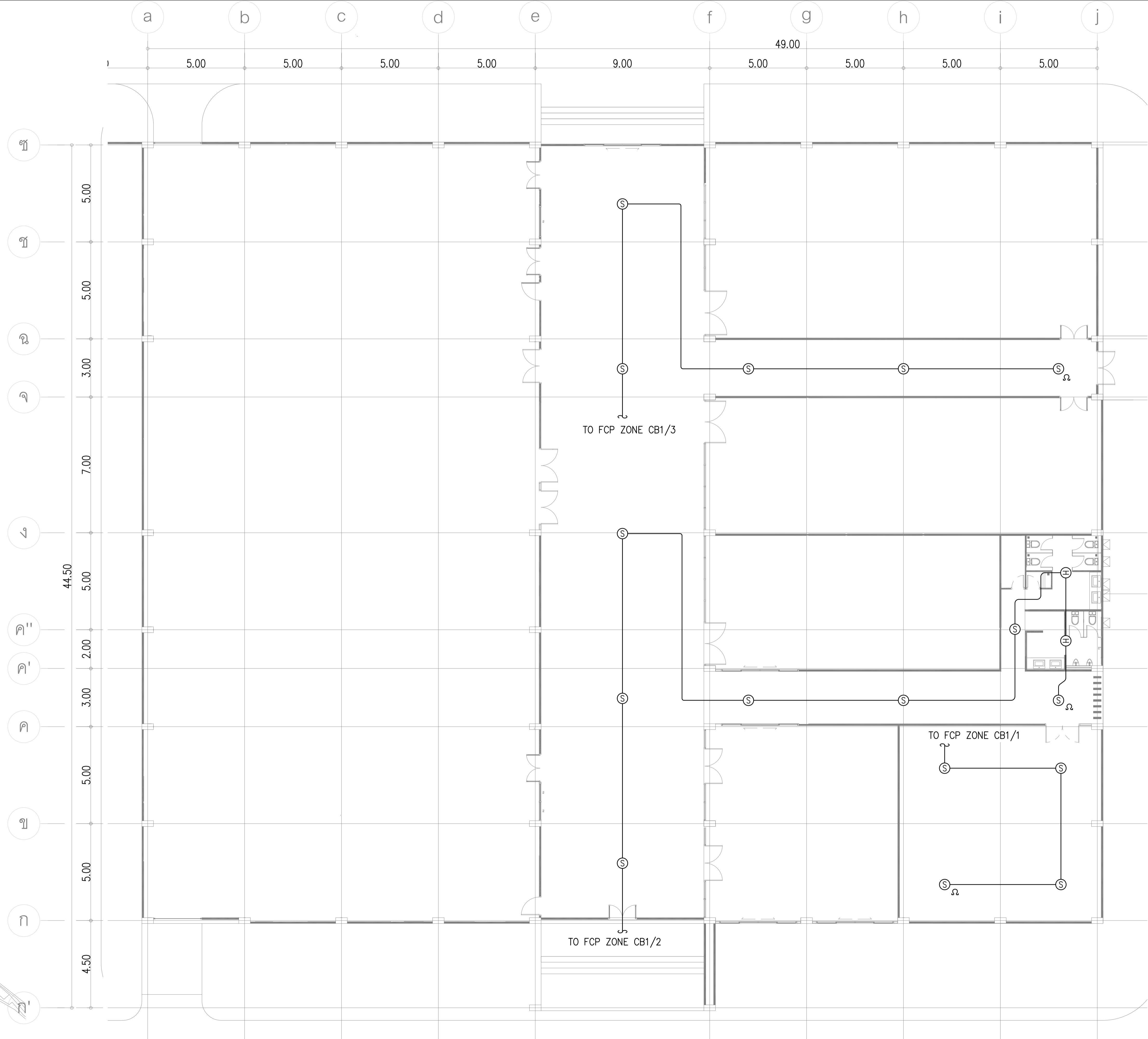
FIRE ALARM, ACCESS CONTROL SYSTEM FOR 1st. FL. (CB1) SCALE 1:100
