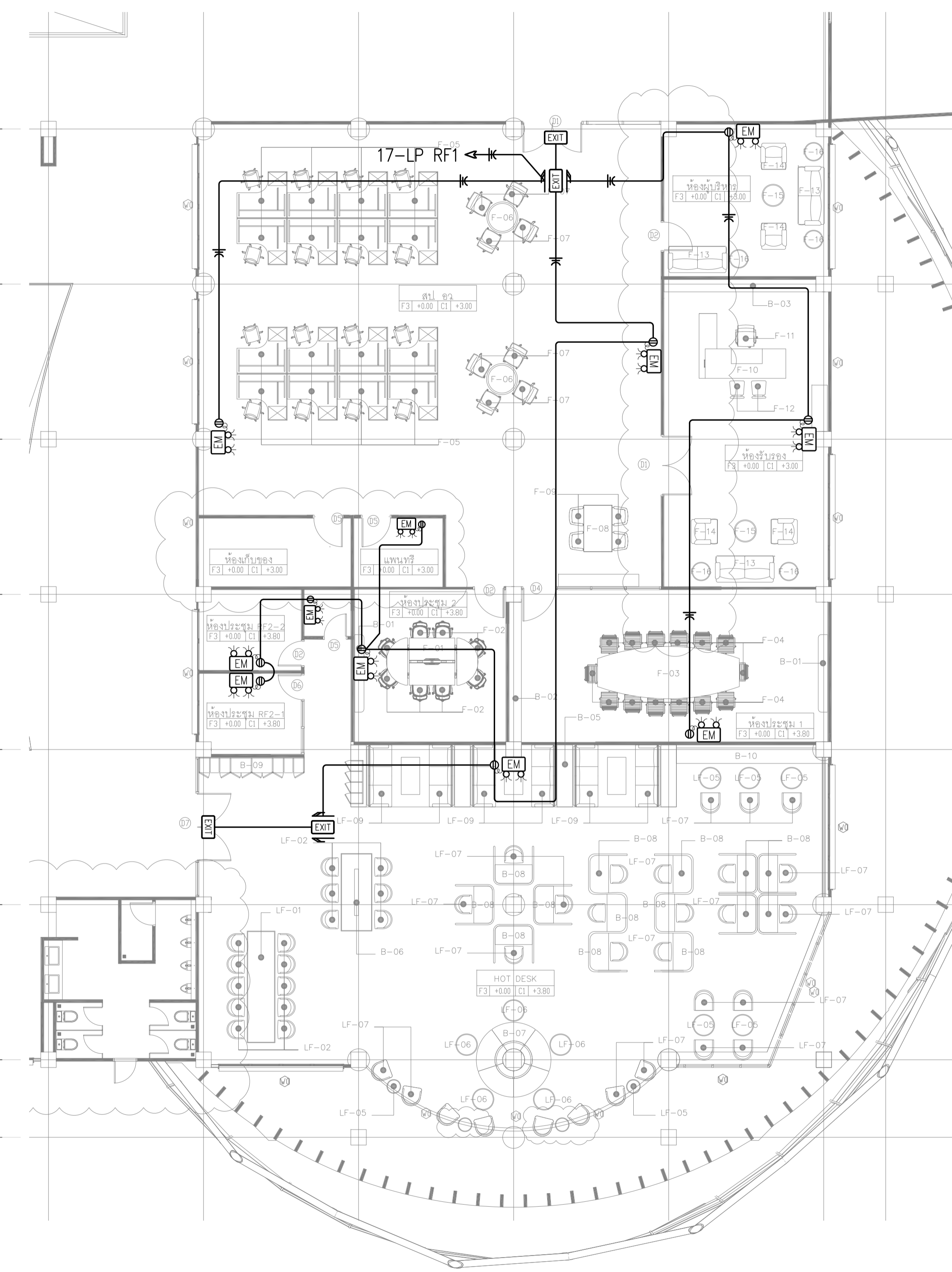
EMERGENCY LIGHT AND EXIT SIGN SYSTEM FOR 2nd. FL. (RF2) SCALE 1:100
