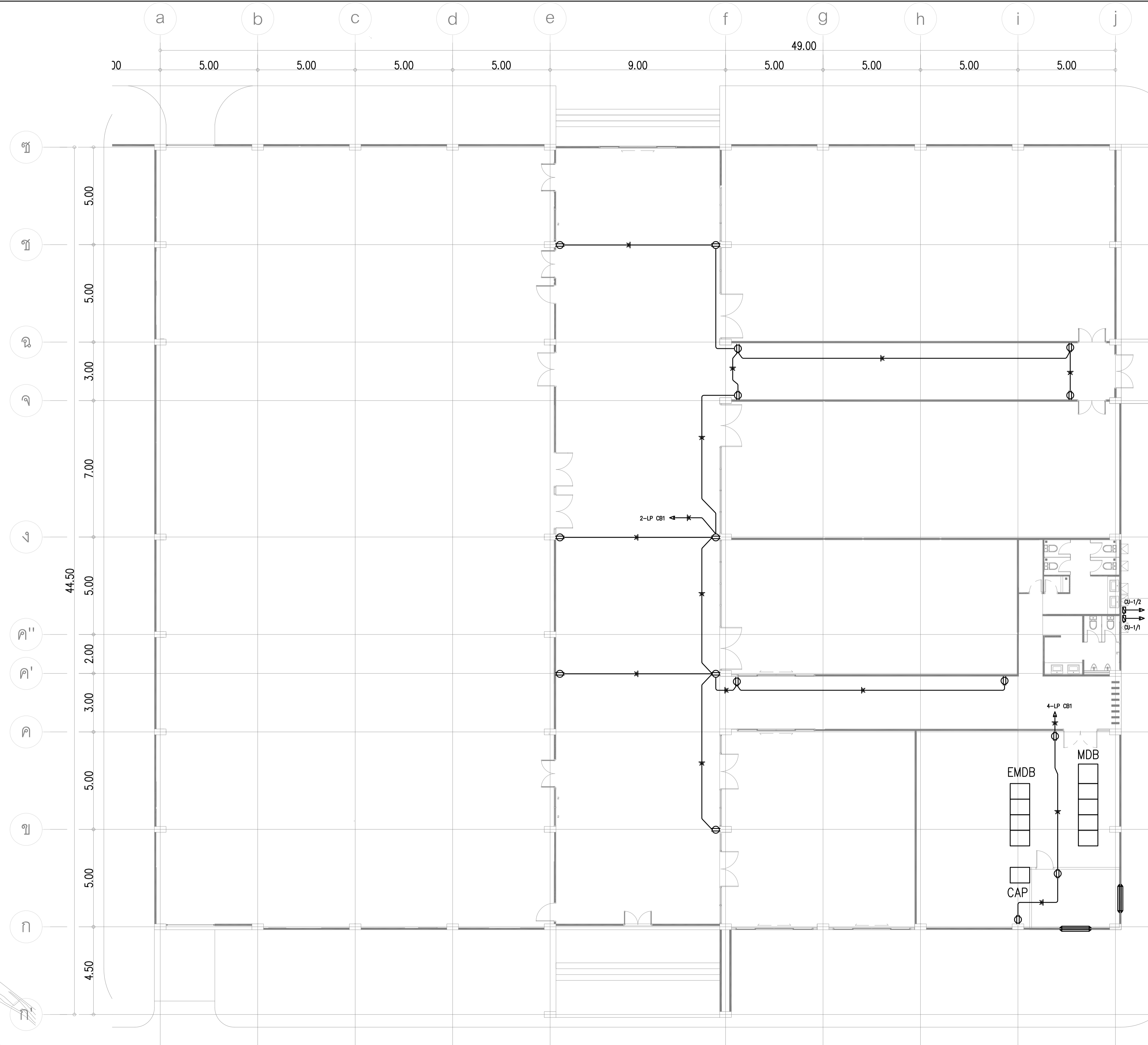
POWER SYSTEM FOR 1st. FL. (CB1)
